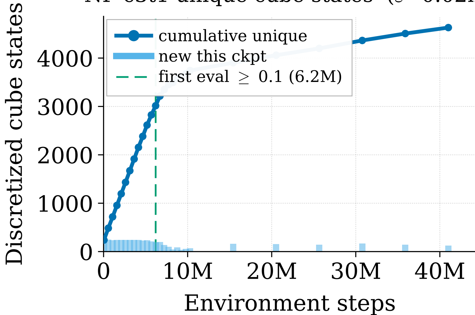
NF c3t1 unique cube states ( \varepsilon=0.02m )
